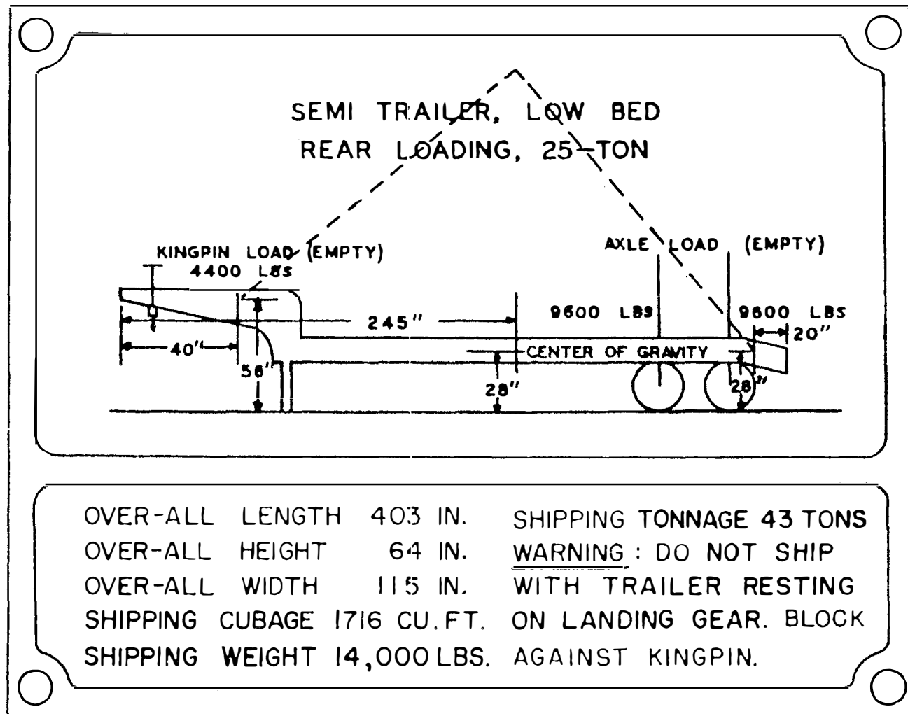
Figure 2. Example of Instruction Plate, Type III.
